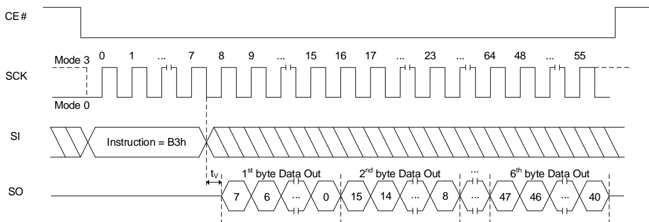
Figure 8.156 Read ECC Register Sequence In SPI Mode
