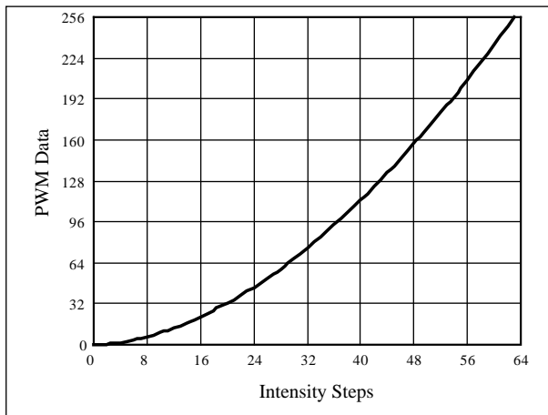
Figure 12 Gamma Correction (64 Steps)
