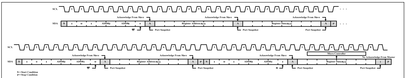
Figure 9 Reading from IS31FL3732A
