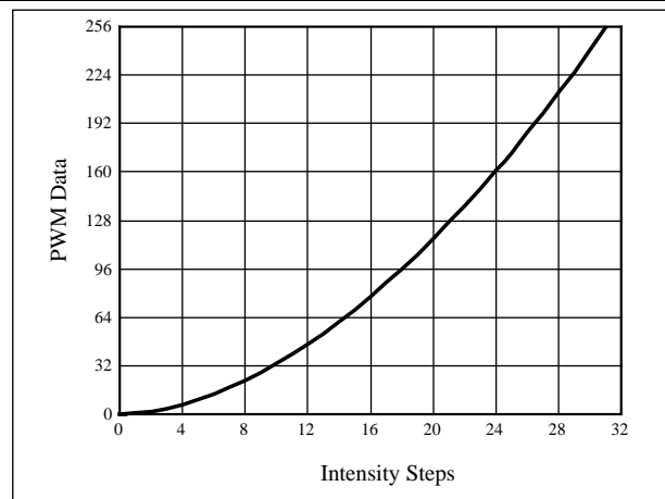
Figure 11 Gamma Correction (32 Steps)
