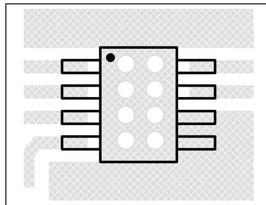
Figure 10 Board Via Layout For Thermal Dissipation
