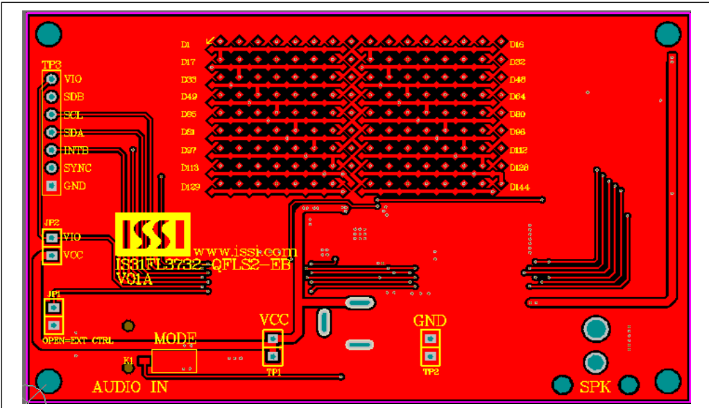
Figure 15: Board PCB Layout - Top Layer
