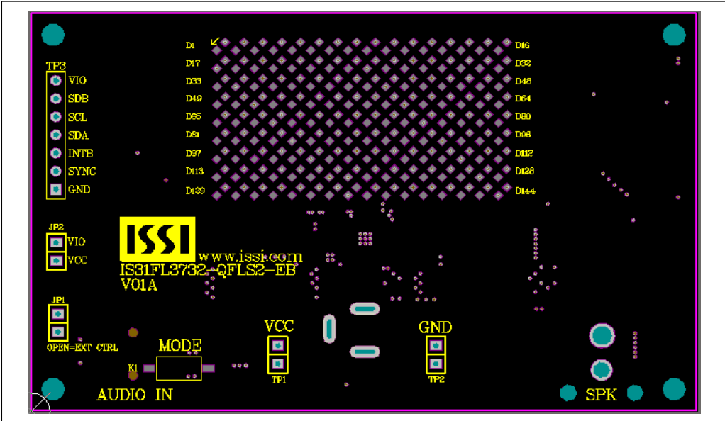
Figure 14: Board Component Placement Guide - Top Layer
