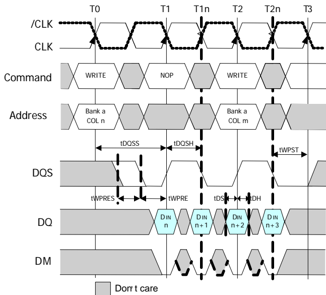
Figure23 : Write Burst (BL=4)
