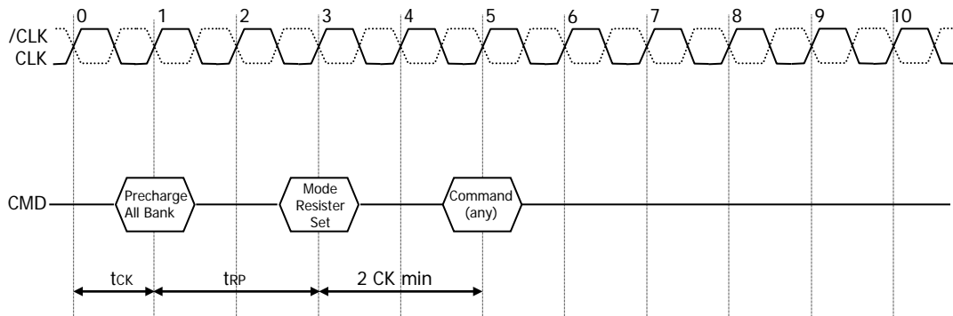
Figure34 : Mode Resister Set
