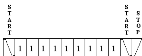
Figure 3: Software reset
