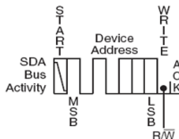
Figure 4: Dummy write operation
