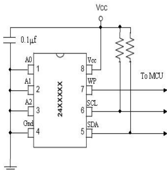
Figure 1: ISSI 24 series EEPROM recommended connections
