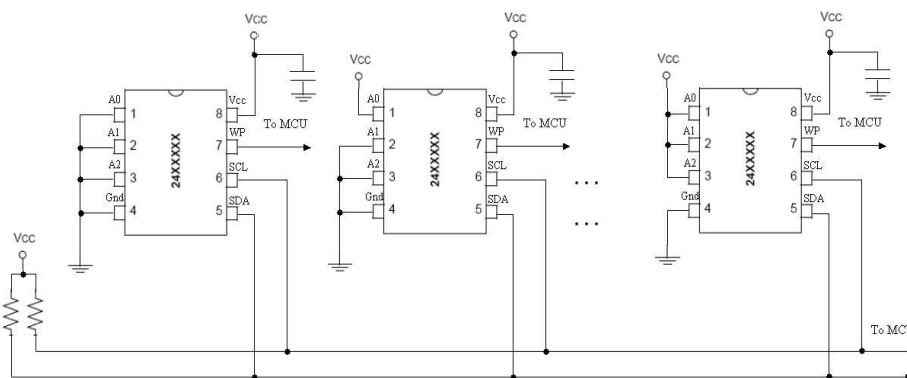
Figure 5: Several EEPROM on a bus
